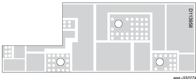
Figure 33. MRF101AN Compact Reference Circuit Board
