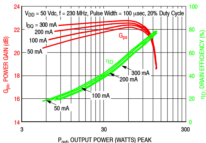
Figure 49. Power Gain and Drain Efficiency versus Output Power and Quiescent Current
